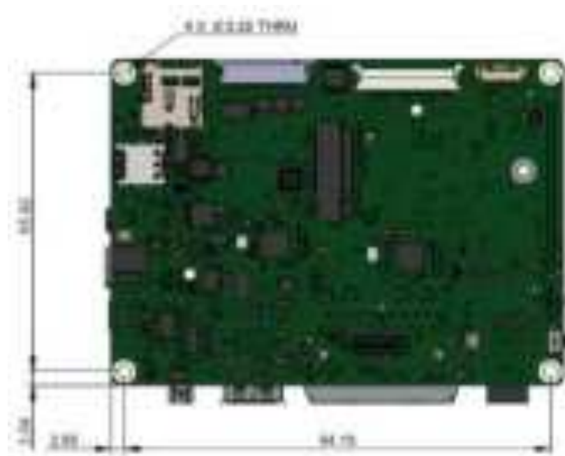
Figure 35: i.MX 8M Plus Pico ITX SBC Mechanical Dimensions Bottom View
